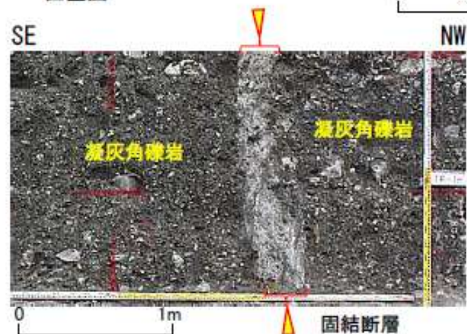
掘削法面② (cf-2断層)
